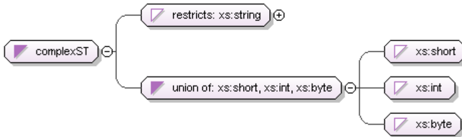
Figure 234. Extracting a Global Simple Type
