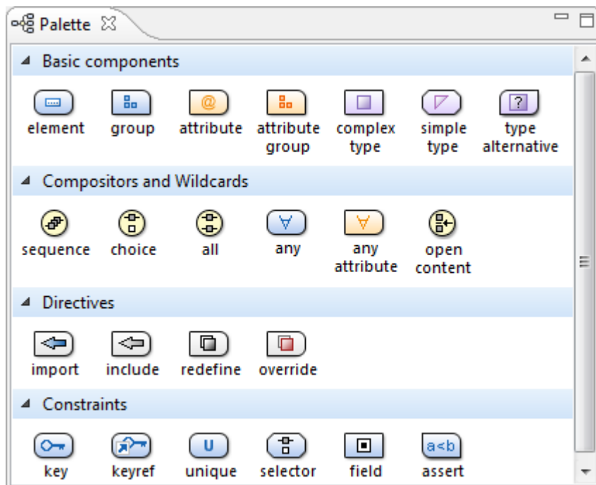
Figure 226. Palette View
