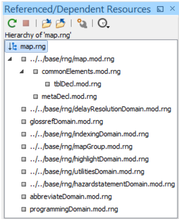
Figure 319. Referenced View
