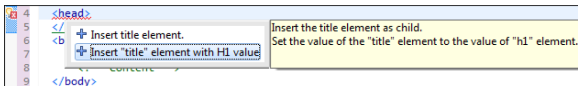
Figure 392. Example of a Schematron Quick Fix
