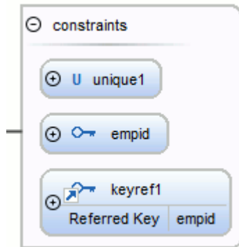
Figure 266. Constraints Construct
