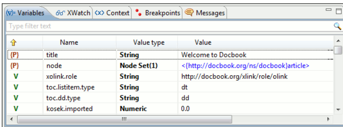
Figure 500. Variables View
