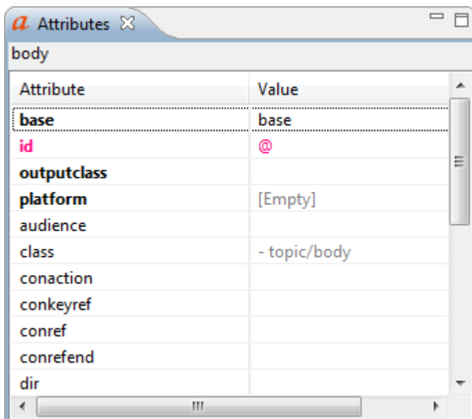
Figure 95. Attributes View
