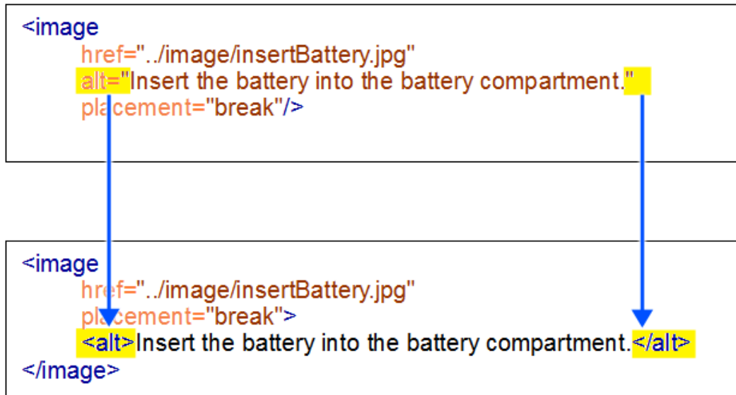
Figure 188. Example: Custom XML Refactoring Operation
