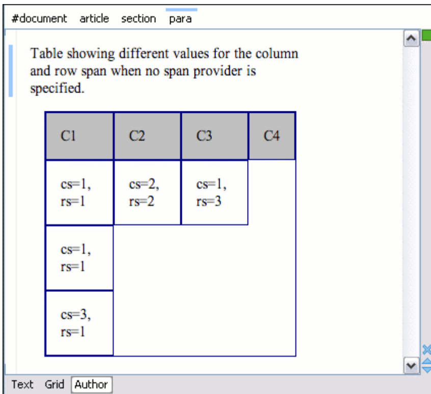
Figure 528. Table layout when no cell span provider is specified
