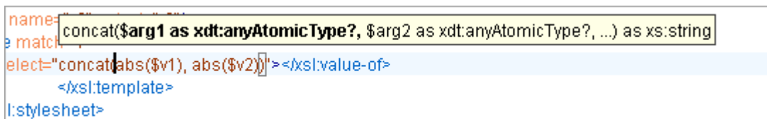
Figure 205. XPath Tooltip Helper - Identify the concat Function's First Argument
