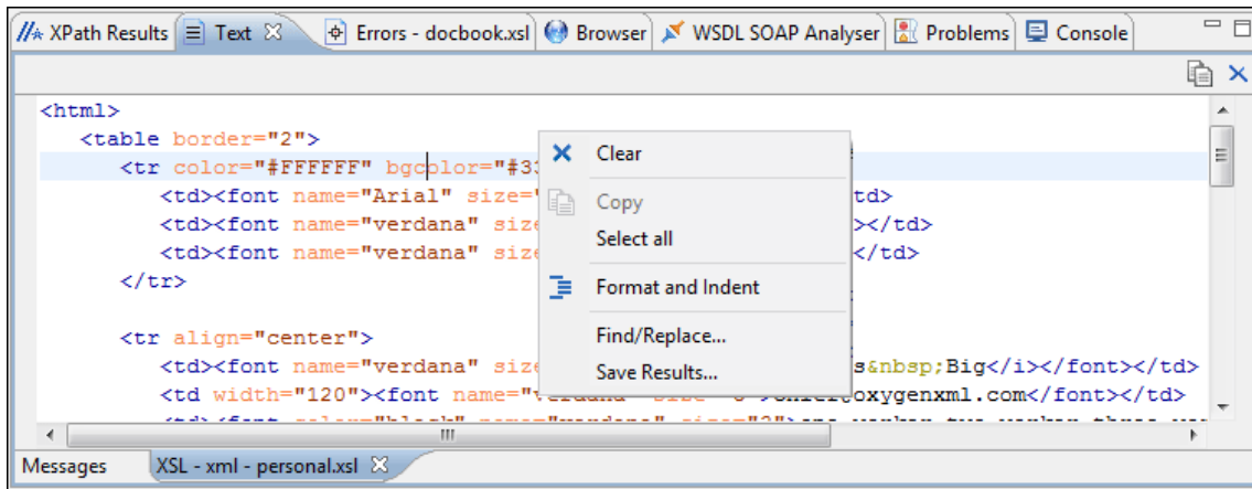
Figure 413. Text View
