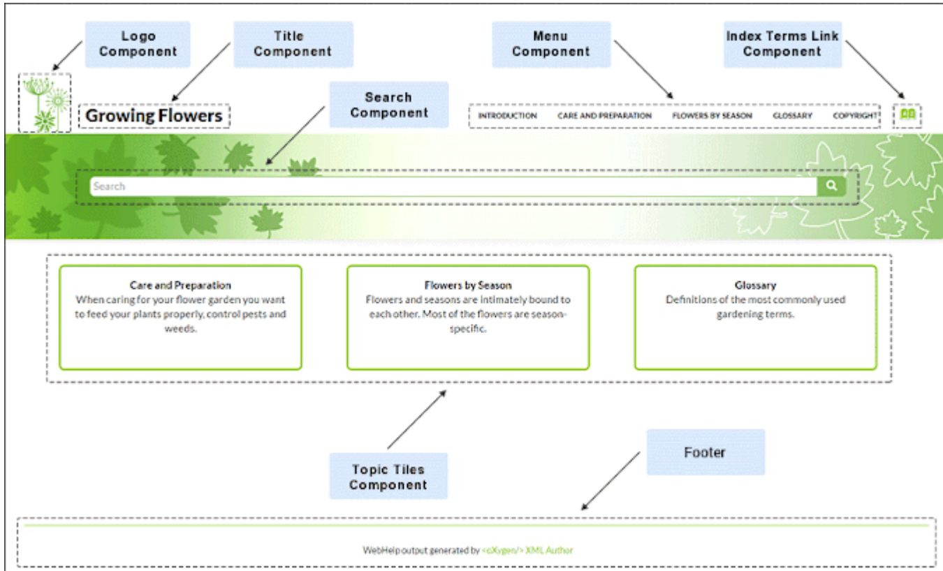
Figure 427. Main Page - Tiles Layout
