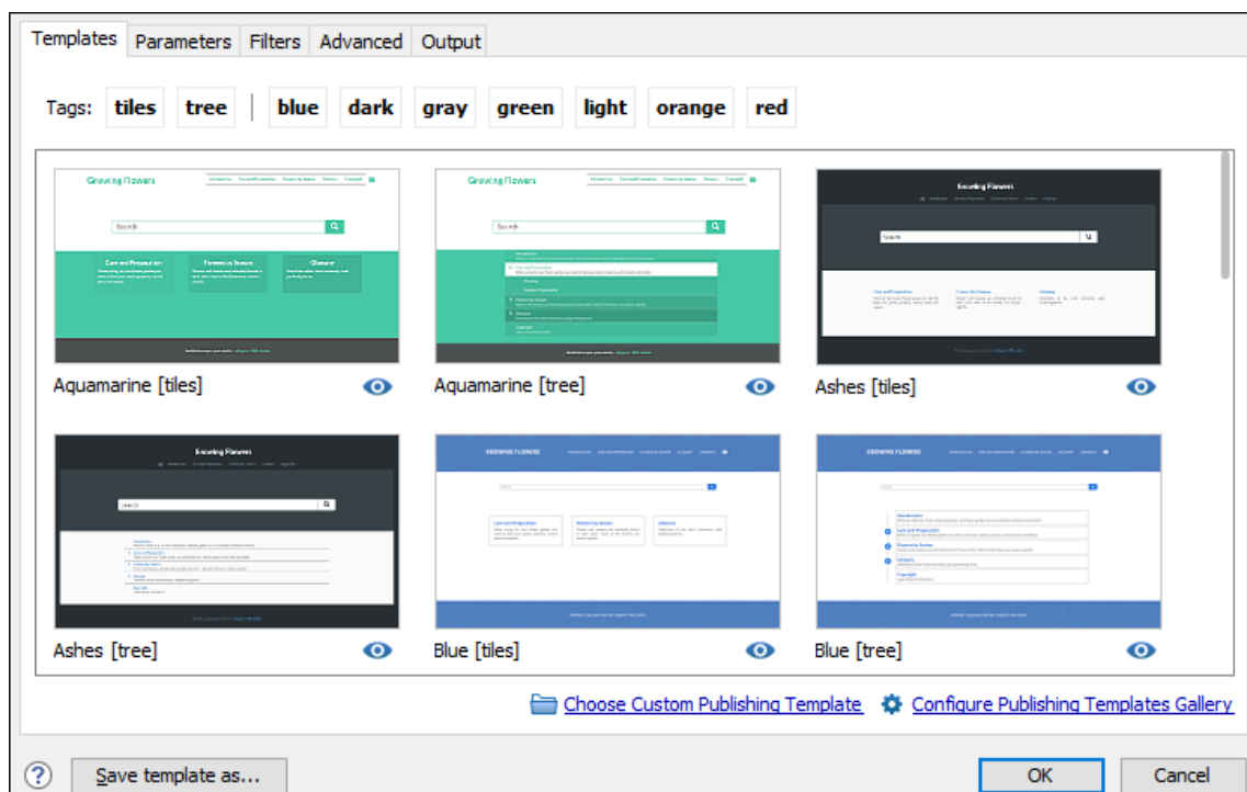
Figure 633. Templates Tab
