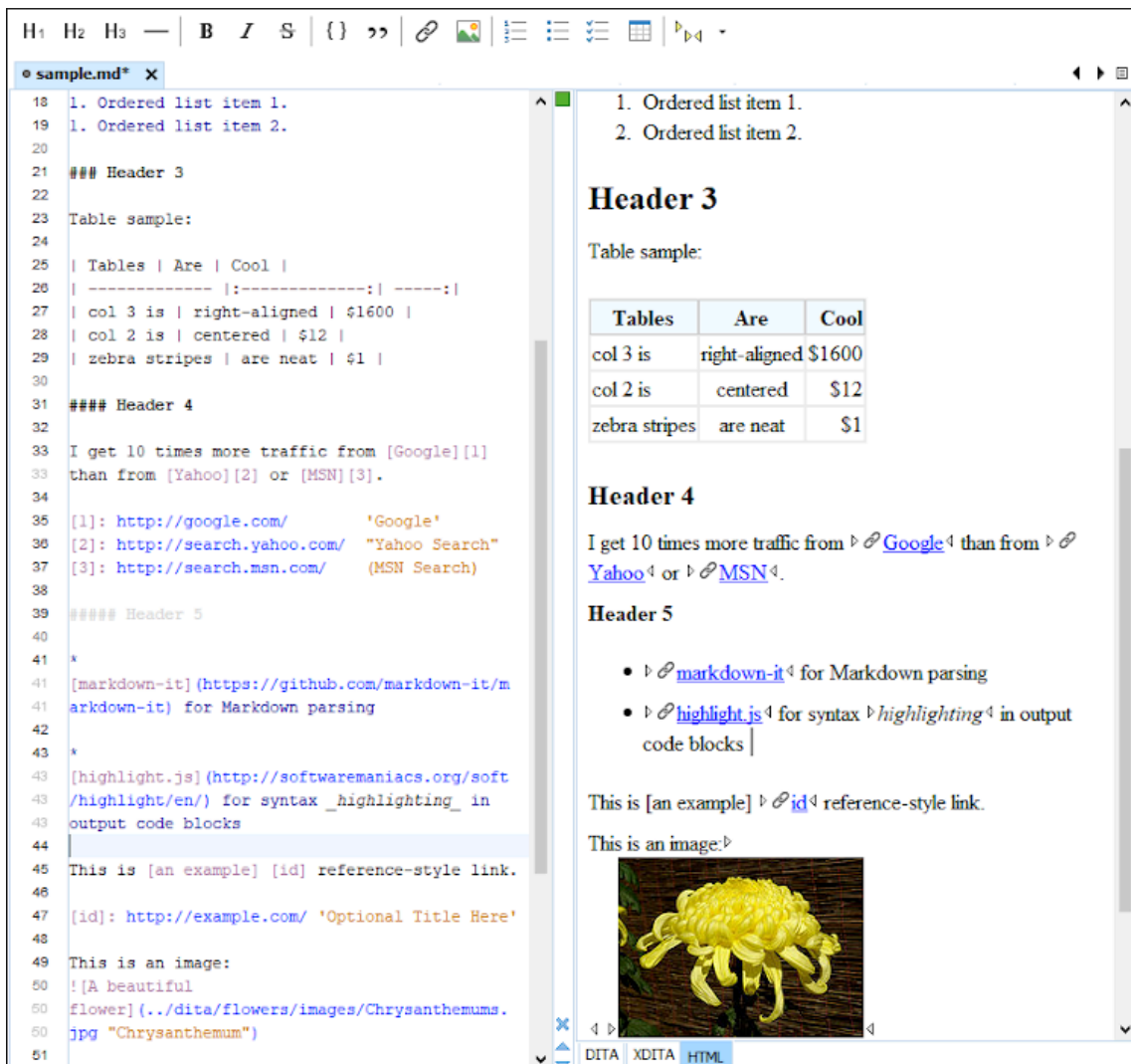
Figure 397. Markdown Editor
