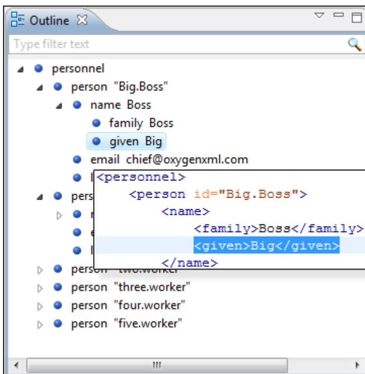
Figure 59. Outline View
