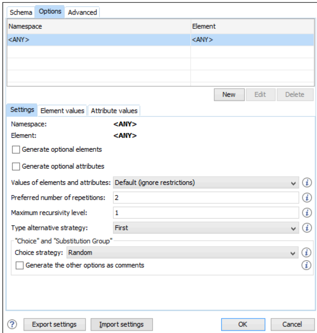
Figure 548. Generate Sample XML Files Dialog Box (Options Tab)
