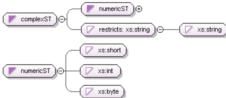
Figure 235. Extracting a Global Simple Type on a union Component
