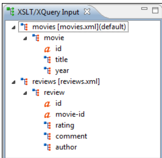
Figure 294. XQuery Input View
